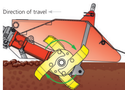
Rotary tilling direction running opposite to the direction of travel
