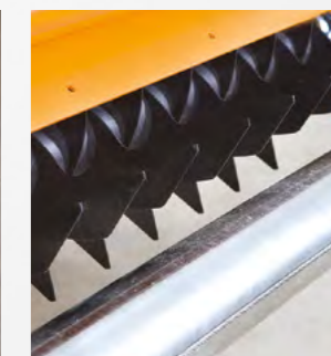
Tungsten tipped 'hook' blades for durability
