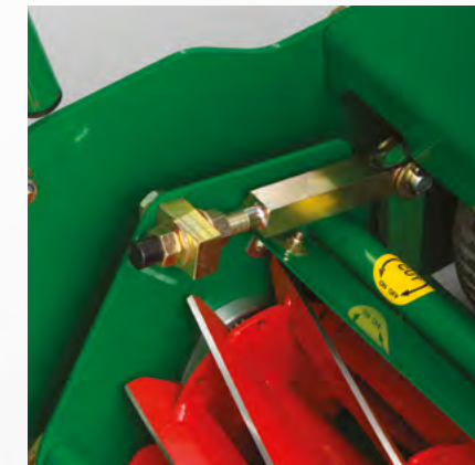
Adjustment of cylinder to bottom blade easy and positive with a single spanner
