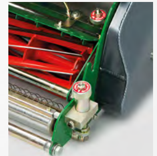
Positive easy height of cut adjustment in 0.25mm increments
