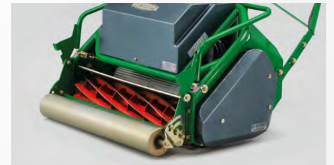
Large diameter front roller with adjustable scraper for precise height of cut control
