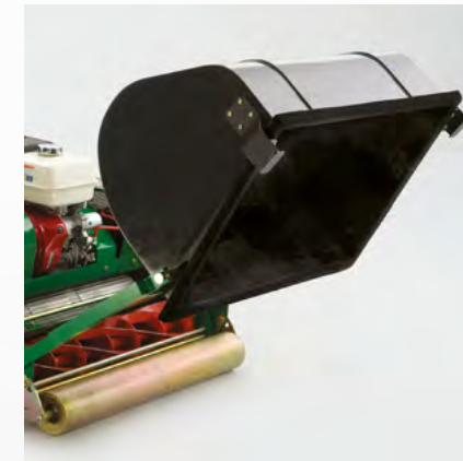
Simple tip over grassbox for easy emptying
