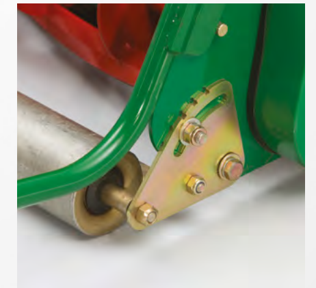
Precise height of cut control which easily adjusts on both sides with a single spanner
